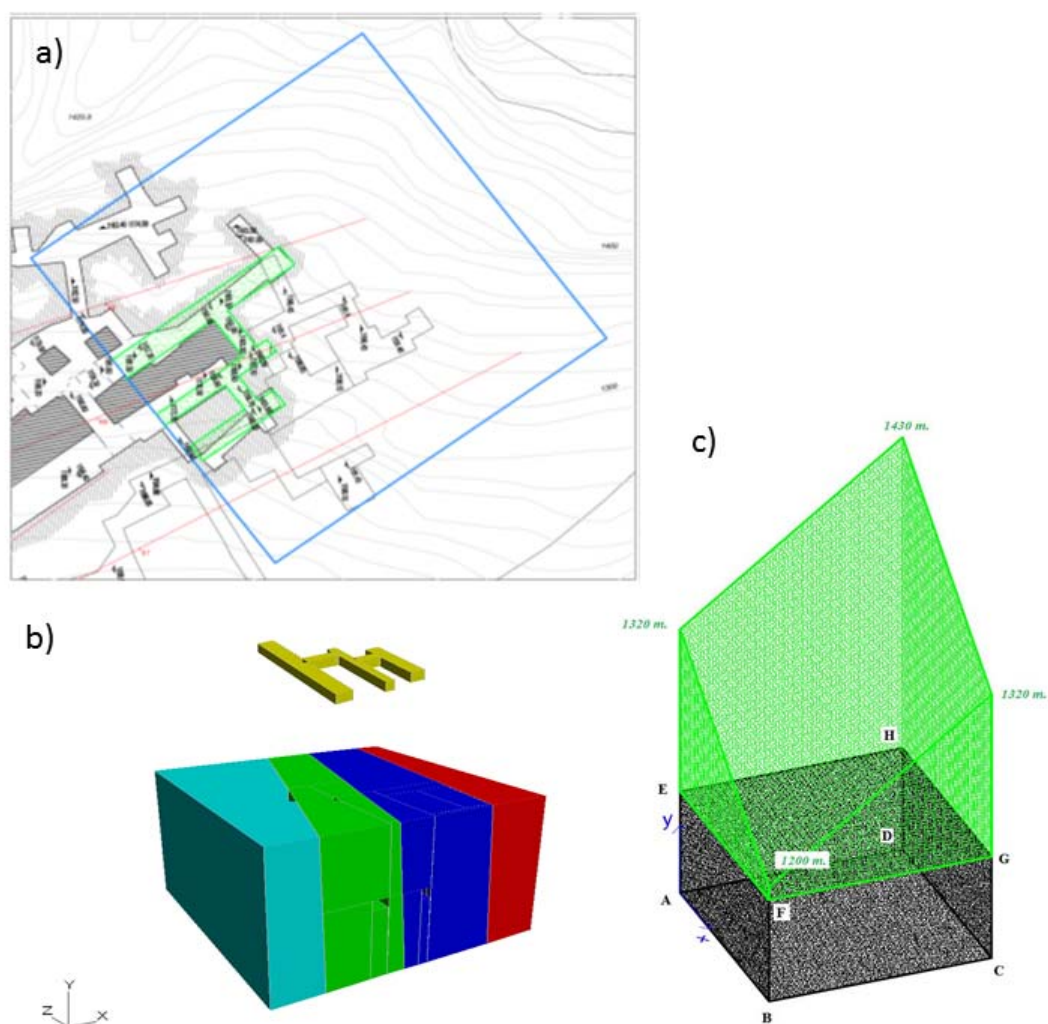
Fig. 12 Analysed portion of the excavation room and its simplification (a); geometric model (b) and load geometry (c).
