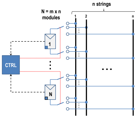
Fig. 3: A Fully Reconfigurable PV Panel.
