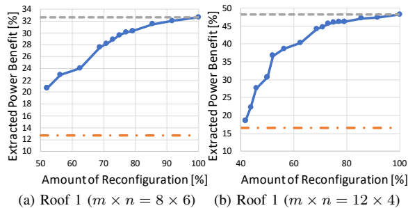
Fig. 9: Results for diode-less panel (Roof 1).
