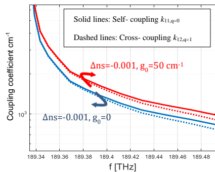
Fig.1 Self- and cross-coupling coefficients of the PhC waveguide
