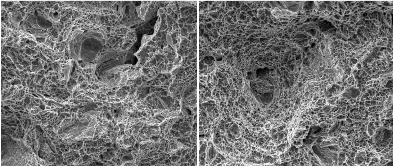
Fig. 11 – Fracture surface of 39NiCrMo3 steel tensile specimens tempered at 220 °C (a) and 240 °C (b). Electron microscopy. Central (normal) part.
