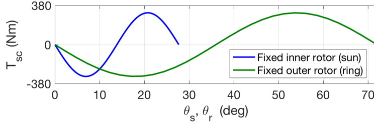
Figure 3: Greyscale map of the sun-carrier torque derived by the simulation of 360 \times 360 relative positions of inner and outer rotor (a). Same torque referred to one period \tau_r or \tau_s while maintaining fixed the position of one of the two rotors (b).
