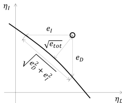
Figure 5 Graphical representation of the derivation of total error. The solid curve is the simplified model, the circle is the reference model data point.
