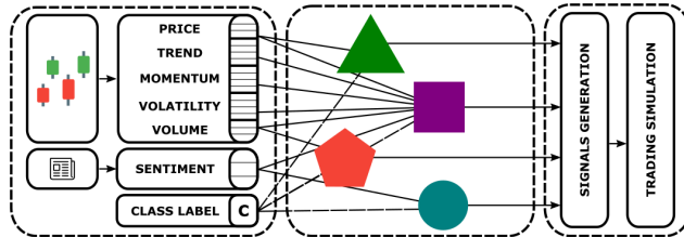
Fig. 1: System architecture.
