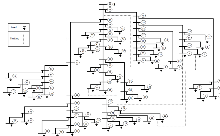
Figure 5. Topological structure considered for the Test90 test case.
