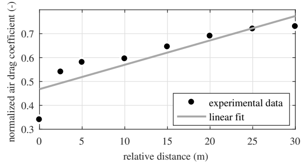
Figure 1. Dependence of the air drag coefficient c_d on the inter-vehicular distance d : experimental data from Hucho (1987) and linear fit.
