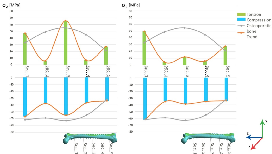
Fig. (3). Average tension (green) and compression (blue) longitudinal stress components \sigma_z for not fractured femur, both in the unplated (grey) and in kissing and overlapped plates configurations (stainless steel (a, c) and titanium alloy (b, d), healthy (a, b) and osteoporotic bone (c, d) during heel-strike phase, in the five cross sections chosen. The orange lines highlight the stresses trend along the diaphyseal axis of the femur in the different configurations.
