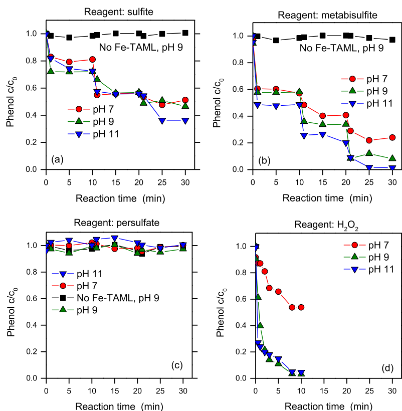
Figure 1. Degradation of phenol with different reagents. Reagents were (a) sulfite, (b) metabisulfite, (c) persulfate, and (d) H_2O_2 . The reactions were carried out in phosphate buffer (10 mM) by adding 0.1 mM of reagent every 10 min (i.e., at t = 0, 10, and 20 min), with the exception of H_2O_2 that was added only once at the beginning ( t = 0 ). Initial conditions were [Fe-TAML] = 0.01 mM; [PhOH] = 0.1 mM.
