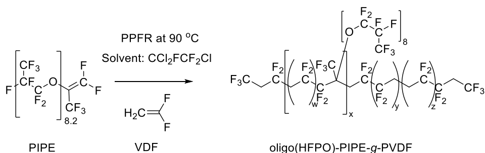
Scheme 3: Radical copolymerizations of oligo(HFPO)-PIPE macromonomer with VDF initiated by \cdot\text{CF}_3 radical generated by PPFR at 90 °C.
