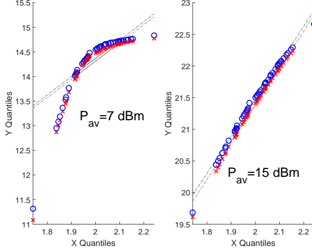
Fig. 4. Q-Q plot of the output power (Y-quantiles) vs. doping (X-quantiles). ADS (blue circles) and TCAD physical analysis (red cross) show a very good agreement. The distribution strongly deviates from the normal one (reference straight line) at low input power.
