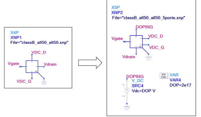
Fig. 2. X-par with extra port DOPING used for interpolation over physical parameters in the X-par file. In this example the original 4-port component (two DC and 2 RF ports) becomes a 5-port: the extra port allows doping dependent analysis.
