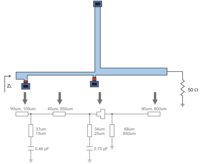
Fig. 7. Layout of the final optimized matching network.
