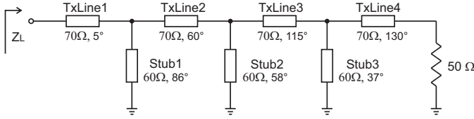
Fig. 5. Tuned load matching network with ideal transmission lines: the matching network controls up to the fifth harmonic.
