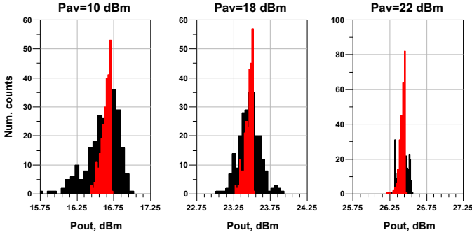
Fig. 10. Output power distribution of the PA stage subject to doping variations (black) and MIM layer variations (red) at different input power levels.
