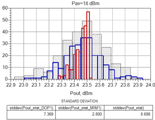
Fig. 11. Output power distribution of the PA stage subject to concurrent doping variations (black) and compared to the separate doping (blue) and MIM layer variations (red).
