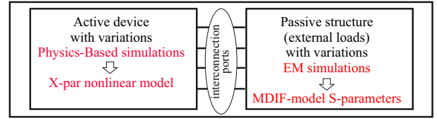
Fig. 1. Multiphysics and multiscale variability analysis of nonlinear stages.
