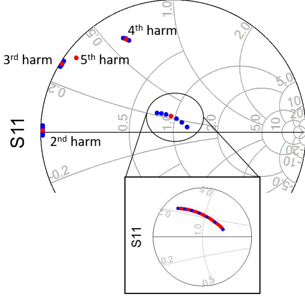
Fig. 8. Variation of the load impedance resulting from a spread of the MIM dielectric thickness. Blue marks: load impedance resulting from EM simulator with a MIM thickness variation of \pm\sigma , \pm2\sigma , \pm3\sigma ( \sigma = 2 nm). Red mark: nominal thickness. In the inset: fundamental frequency impedance. Blue marks: EM simulations as before, used for the MDIF dataset. Red line: ADS MDIF interpolated model with the MIM thickness varying between 94 and 106 nm.
