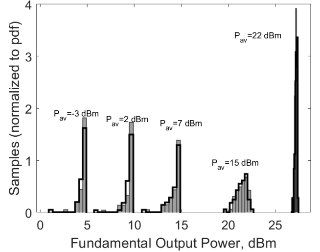
Fig. 3. Histograms of the output power (dBm) of the class AB stage as a function of random doping variations at varying input power. Shaded: ADS Monte Carlo analysis with 50 samples. Solid lines: TCAD Monte Carlo analysis carried out on the same doping samples.
