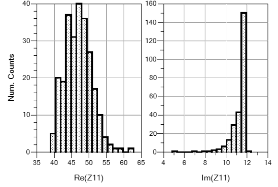
Fig. 9. Real and imaginary parts of the load impedance resulting from a random MIM layer thickness with a Gaussian distribution of 2% standard deviation.
