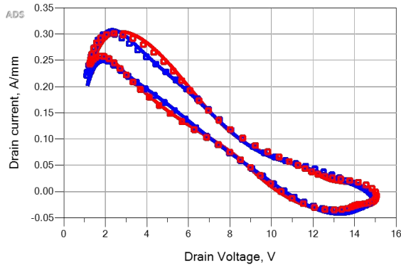
Fig. 6. Comparison of the DLL lines on the ideal optimum load (blue) and on the loads synthesized by the matching network of Fig. 5 (red). Solid lines: ADS X-par model. Symbols: Physics-based TCAD simulations. The input power is 22 dBm, driving the device well into compression.
