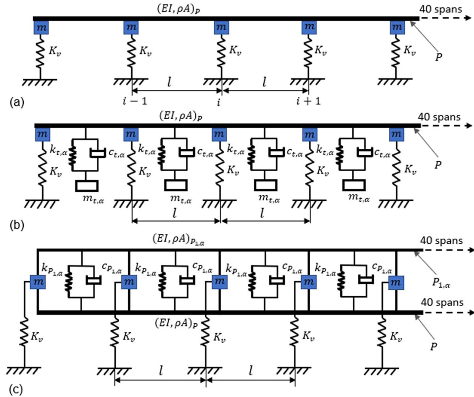
Figure 2. Models for a pipe P of Fig. 1b on a periodic rack, i.e. a pipe on elastic supports- Type #2-. (a) Uncontrolled pipe P . (b) Pipe P with lateral localized resonator (LLR) at the centre of each unit cell. (c) Pipe P connected to lateral distributed resonator (LDR), i.e. pipe P 1,α .
