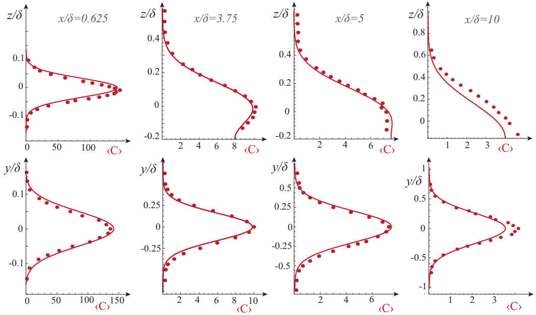
FIG. 7. Mean plume spread for the elevated sources ES6. Notice that, as the mean is affected by the source diameter just in proximity of the source, there is no need to discriminate between ES3 and ES6 [38].
