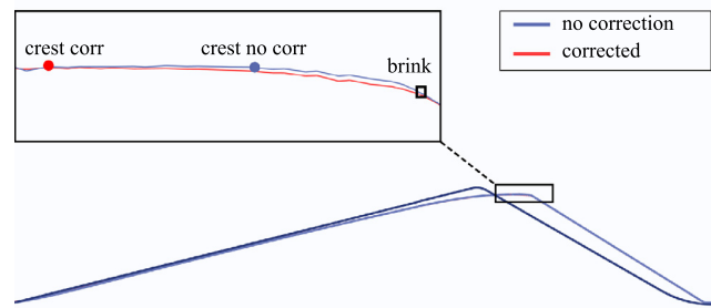
Fig. 9. Comparison of the dune configuration at t = 600 s with and without the slope-sensitive u_t^* model correction; that is, Eq. (4). The zoomed panel highlights the crest-brink separation obtained with the modified model.
