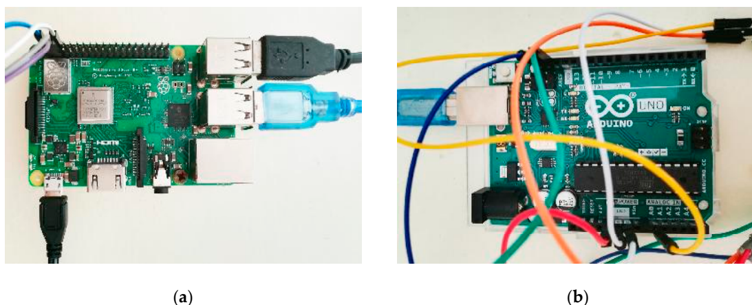
Figure 2. (a) a view of the master unit used (Raspberry Pi 3B+) (b) one the used slave unit board used (Arduino UNO R3).
