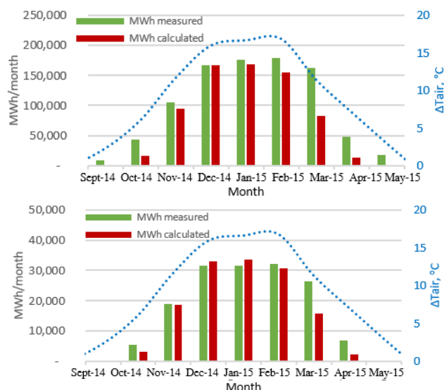
Figure 9. Comparison between the monthly measured and the forecast consumptions for the 2014-15 heating season using scale ‘3’ (Figure 6): a) H+DHW; b) H
