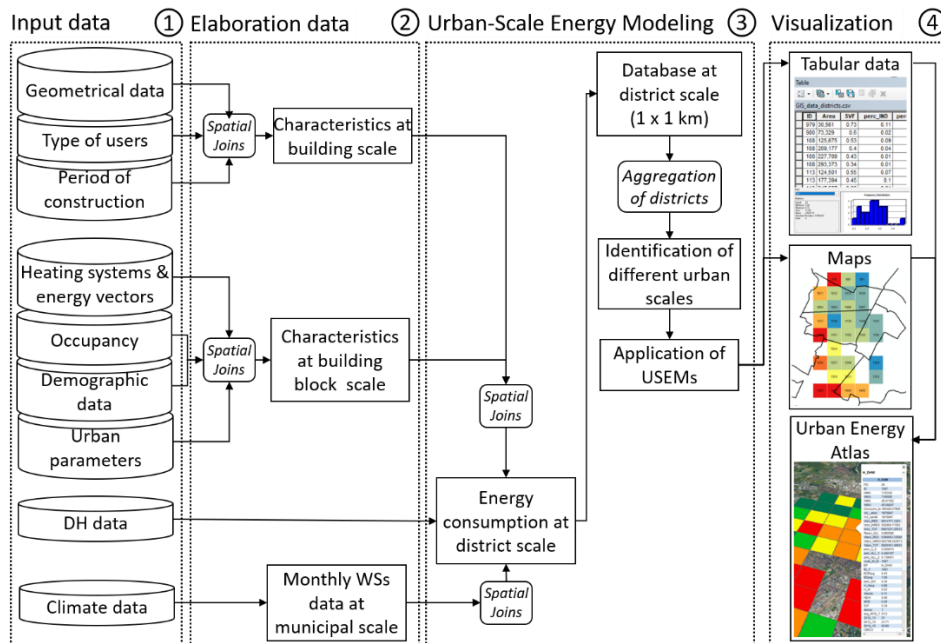
Figure 3. Flowchart of the urban energy atlas methodology
