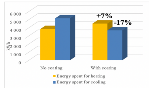
Fig. 3. Total energy consumption comparison between “No coating” and “With coating” scenarios.
