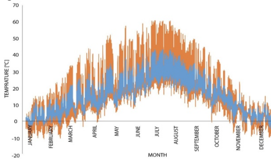
Fig. 2. Roof surface temperature comparison with (blue curve) and without (orange curve) the white coating over a year.
