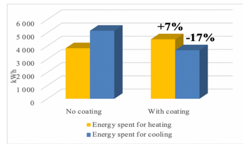
Fig. 3. Total energy consumption comparison between “No coating” and “With coating” scenarios.
