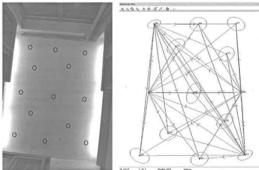
Fig. 2. Reference system – circles evidence the markers (left), Least Square network adjustment with error ellipses (right).
