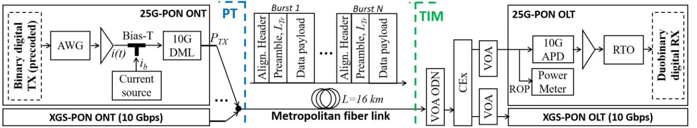
Fig. 4 Metropolitan field demonstrator setup.
