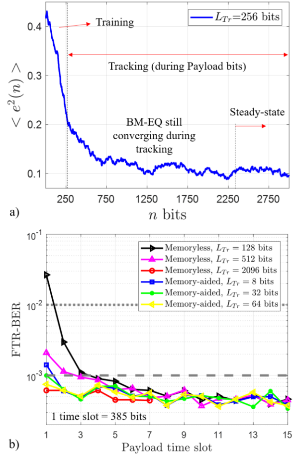
Fig. 10 a) Error square evolution over time for a given L_{Tr} ; b) FTR-BER over each of the 385-bit time slots for memory-aided and memoryless BM-AE approaches with different training length L_{Tr} . ODN loss = 28.7 dB.
