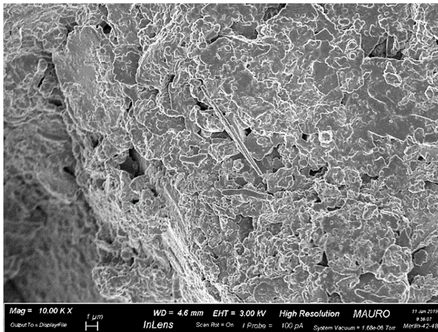
Figure 6. SEM image of aerated column sample (bottom). The diesel coating is evident. Magnification: 10,000×.
