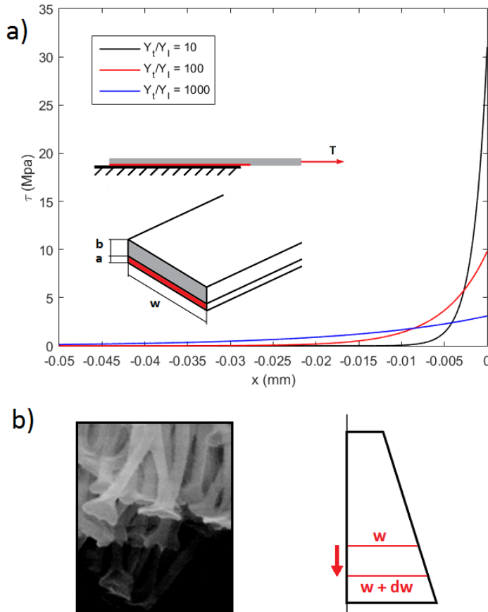
Figure 7-6: a) Geometry of the considered a thin elastic layer with a “ventral” soft interface and an applied horizontal force T . Shear stress distributions are plotted along the length of the attached region for varying ratios between contact layer stiffness Y_l and tape stiffness Y_t . Softer contact layers are shown to reduce stress concentrations with respect to stiffer layers. b) tapered geometry of terminal contact element width to increase peeling line ( w \rightarrow w+dw ) during delamination (image from [25])
