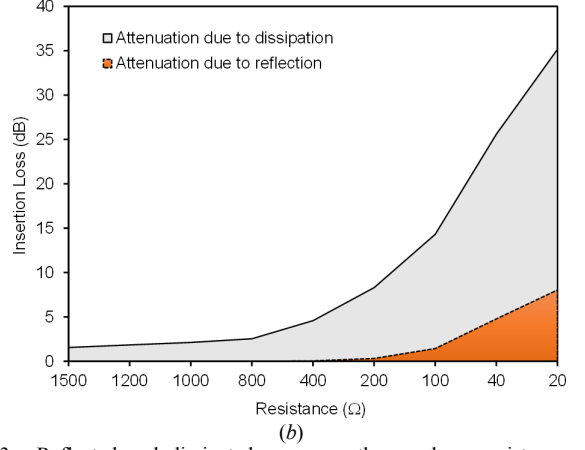
Fig. 3. Reflected and dissipated power vs the graphene resistance at the frequency of 5 GHz: (a) simulated results for the 2-post design; (b) simulation results for the 4-post design.
