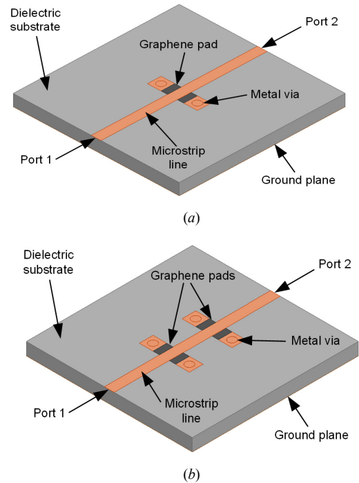
Fig 1. Geometry of the graphene-based tunable microstrip attenuators: (a) Microstrip attenuator with one pair of symmetrical graphene pads, located between the microstrip line and grounded vias; (b) Microstrip attenuator with two pairs of graphene pads, spaced by a microstrip line section.
