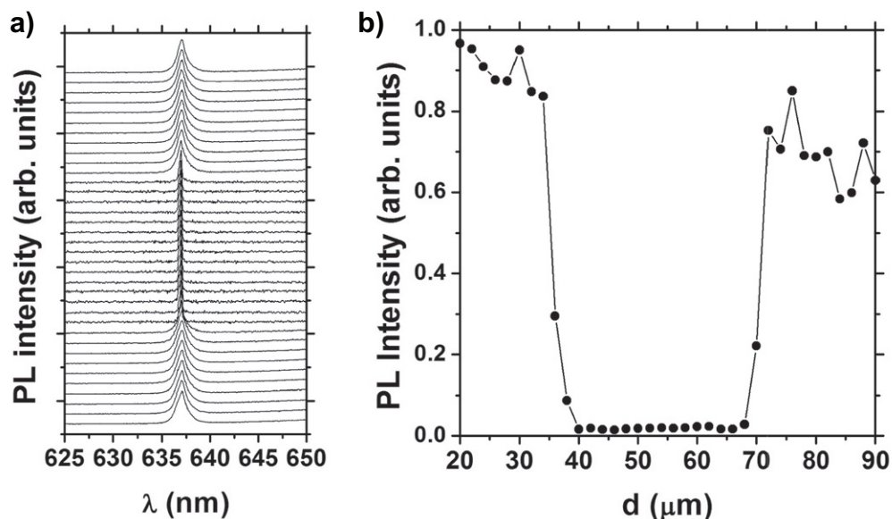
Figure 10. (a) normalized PL spectra collected at 2 \mu\text{m} steps away from the implanted region and across the low-nitrogen ‘edge’ sector (see the blue arrow in figure 2); the spectra are displaced along the vertical axis for readability; (b) intensity of the ZPL \text{NV}^- emission along the linear scan; the extension of the ‘edge’ sector can be clearly distinguished by the significant sharpening (a) and the decrease in intensity (b) of the \text{NV}^- emission.
