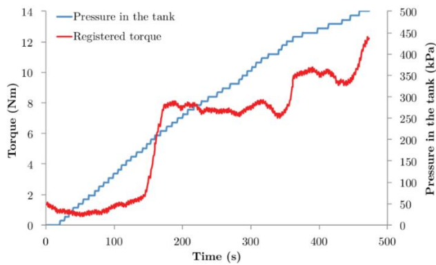
Fig 7 Measured torque on the blades increasing the pressure on a sand ( D_{10}=0.1\text{mm} ; D_{60}=0.2\text{mm} ) conditioned with \text{FER}=15 ; \text{FIR}=80\% , c_f=2\% and w=20\% [38].
