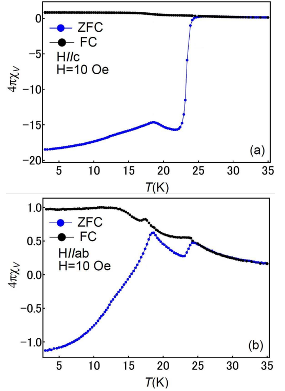
FIG. 9. Temperature dependence of external volume susceptibility in a 10 Oe field applied parallel to c axis (a) and to ab planes (b), measured by a SQUID magnetometer.
