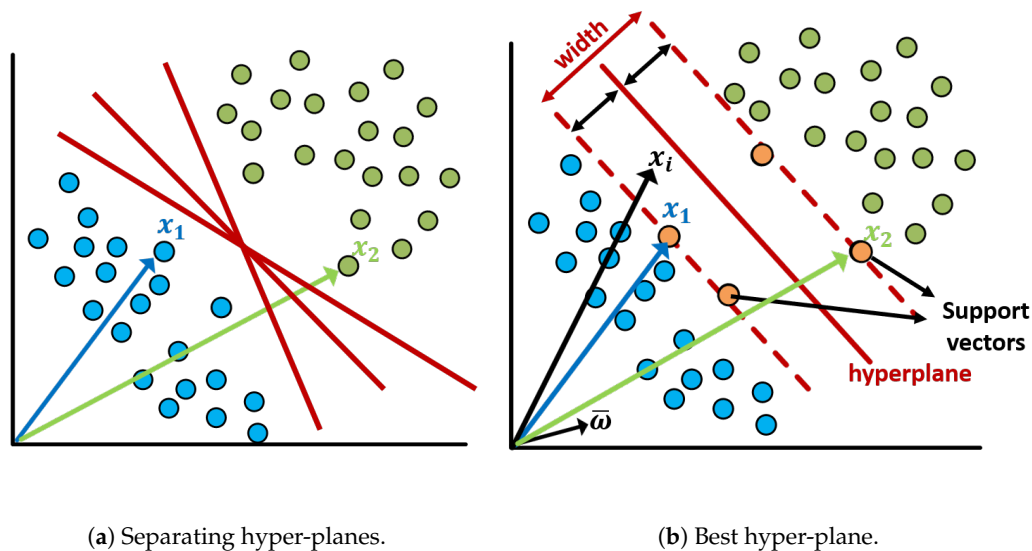
(a) Separating hyper-planes. (b) Best hyper-plane. Figure 4. An overview sketch of Support Vector Machines (SVM) algorithm linear classifier.
