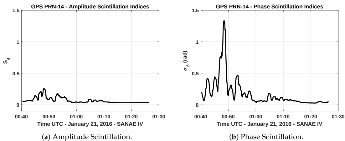
Figure 2. Scintillation index values of GPS L1 C/A PRN-14 signal—21 January 2016 (SANA IV).
