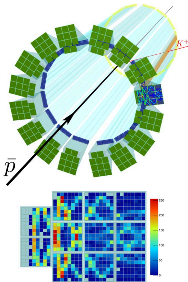
Figure 14. Geant simulation of the baseline geometry of the \bar{\text{PANDA}} Barrel DIRC. The colored histogram at the bottom shows the accumulated hit pattern from 1000 K^+ at 3.5 GeV/c momentum and 55^\circ polar angle, the red line shows the kaon trajectory. (Top) Reproduced from 2018 JINST 13 C03004. © 2018 IOP Publishing Ltd and Sissa Medialab srl. All rights reserved. (Bottom) Reproduced from 2017 JINST 12 C07006. © 2017 IOP Publishing Ltd and Sissa Medialab srl. All rights reserved.
