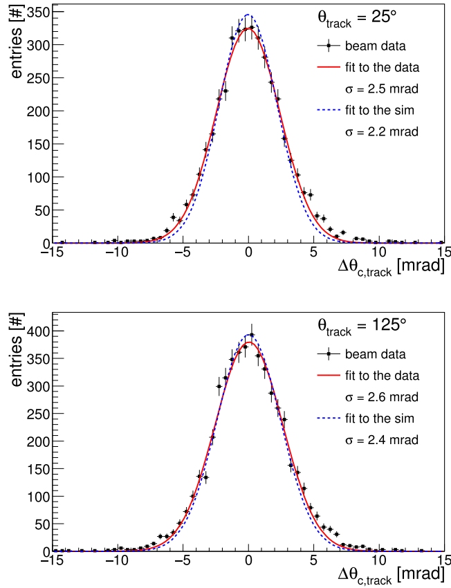
Figure 101. Resolution of the reconstructed Cherenkov angle per track for proton tags (data) and protons (simulation) with a momentum of 7 GeV/ c , a polar angle of 25° (top) and 125° (bottom). The narrow bar with the 3-layer spherical lens is used.
