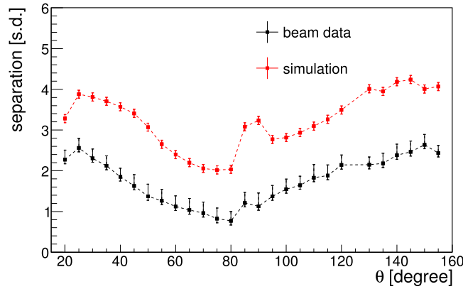
Figure 111. Proton/pion separation power from time-based imaging as the function of the polar angle at 7 GeV/ c momentum for the wide plate without focusing in the beam data (black) and the simulation (red), assuming 100 ps time resolution and a 3 mm RMS beam spot (red).
