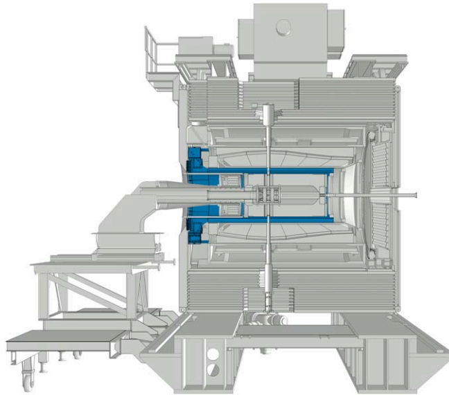
Figure 137. Cross section of the \bar{\text{P}}\text{ANDA} target spectrometer with the Barrel DIRC marked in blue. The auxiliary platform used for detector installation is seen on the left. Reproduced from 2018 JINST 13 C03004. © 2018 IOP Publishing Ltd and Sissa Medialab srl. All rights reserved.
