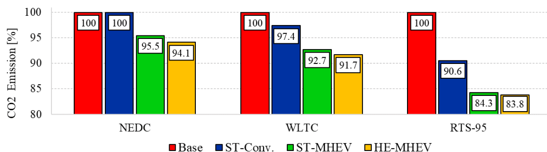
Figure 10. Normalized CO 2 emissions for the NEDC, WLTC and RTS-95.
