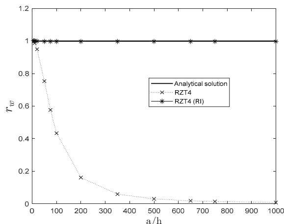
Figure 11. Shear-locking effect analysis for RZT4 element using full and reduced integration. Laminate L. Mesh 8 × 8 of a quarter of the plate.
