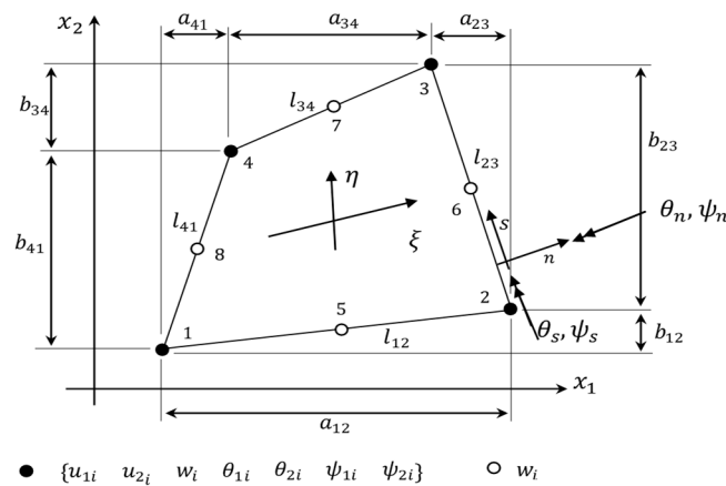
Figure 4. Eight-node virgin quadrilateral plate element. Geometry, physical co-ordinates ( x_1, x_2 ), and natural co-ordinates ( \xi, \eta ). Boundary co-ordinate system ( n, s ). Definition of the parameters a_{ij} and b_{ij} entering in Equations (56) and (63) and the positive rotations ( \theta_1, \theta_2 ) and ( \theta_n, \theta_s ).
