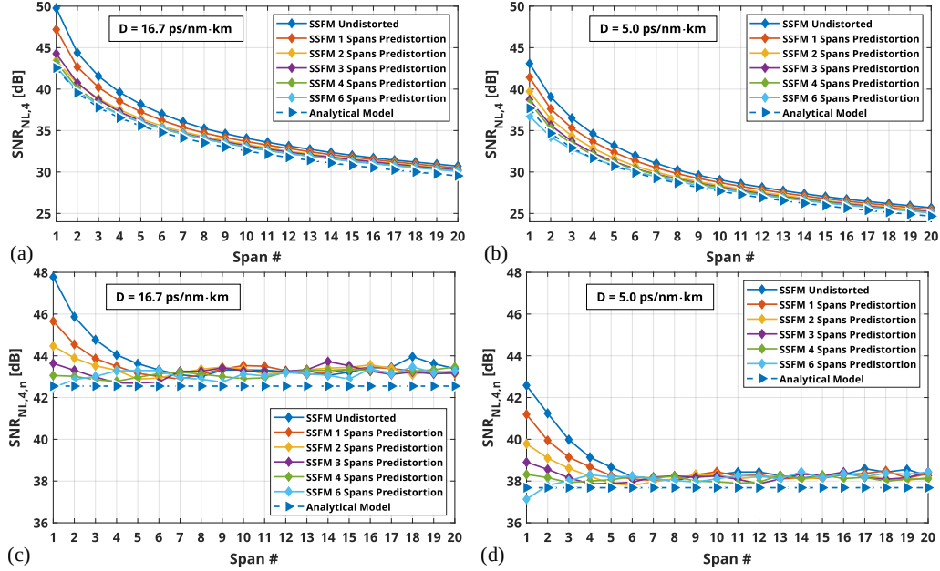
Fig. 2: SNR_{NL} accumulation along the fiber spans simulated by SSFM with applied predistortion of 0 to 6 spans and estimated by the analytic model for (a) D = 16.7 ps/(nm·km), (b) D = 5 ps/(nm·km). Corresponding SNR_{NL} degradation introduced by each span for (c) D = 16.7 ps/(nm·km), (d) D = 5 ps/(nm·km)
