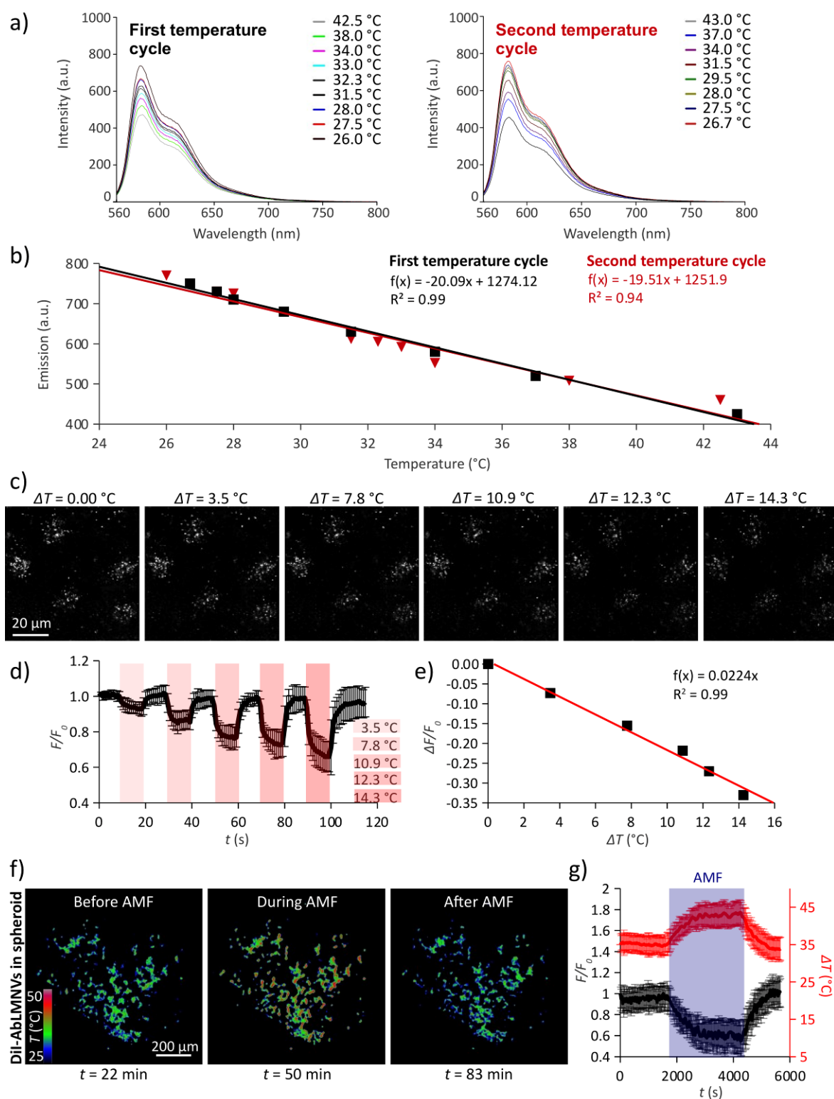
Figure 6. Intraparticle temperature monitoring during AMF stimulation. a) Thermosensitivity of fluorescence of the Dil dye in DMSO; fluorescence emission of Dil during two temperature cycles, shown in the left and right graph, respectively. b) Linear dependency between the Dil fluorescence emission peak (at \lambda = 583 \text{ nm} ) and the temperature during the two temperature cycles (respectively shown in black and in red). c) Fluorescence imaging of the Dil-labeled AbLMNVs during heating ( \Delta T_1 = 0.0^\circ\text{C} ; \Delta T_2 = 2.4^\circ\text{C} ; \Delta T_3 = 5.4^\circ\text{C} ; \Delta T_4 = 7.5^\circ\text{C} ; \Delta T_5 = 8.6^\circ\text{C} ; \Delta T_6 = 9.9^\circ\text{C} ) induced by an infrared (IR) laser source. d) Fluorescence intensity ( F/F_0 ) of the Dil-labeled AbLMNVs during heating. e) Linear relation between \Delta F/F_0 and \Delta T in Dil-labeled
