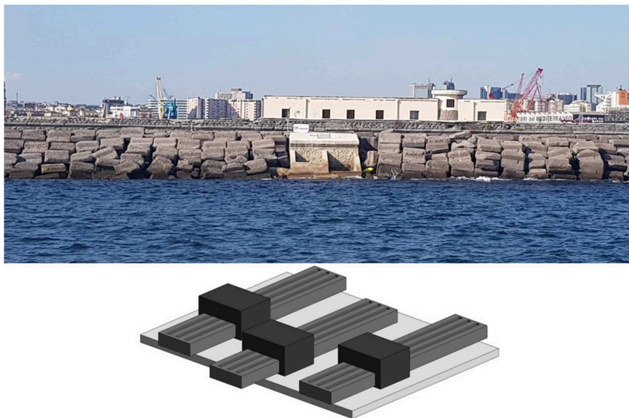
FIGURE 9 | Full scale OBREC in the port of Naples (Top) . Schematic representation of a 40 South Energy H24 wave energy converter plant (Bottom) .
