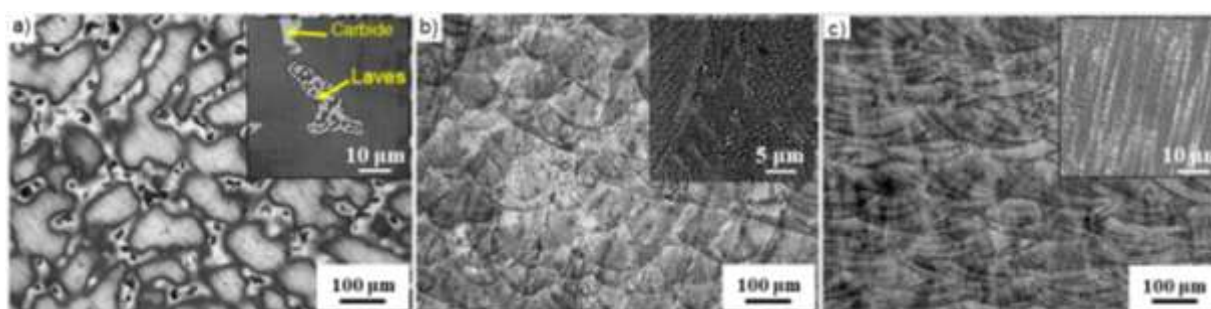
Figure 2 OM micrograph of IN718 alloy in (a) as-cast, (b) as-built LPBF, (c) as-built DED conditions.
