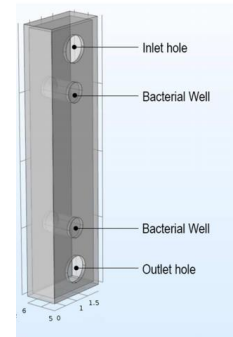
Fig. 4: Sample chamber. The dimensions are measured in [m]
