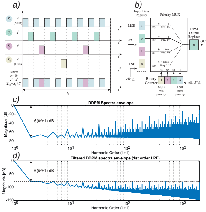
Fig. 3. Dyadic Digital Pulse Modulation (DDPM) [15]: a) DDPM pattern, b) DDPM modulator hardware, c) envelope of the spectra of the 4096 12-bit DDPM patterns, d) spectral envelope as in c) after first-order filtering.
