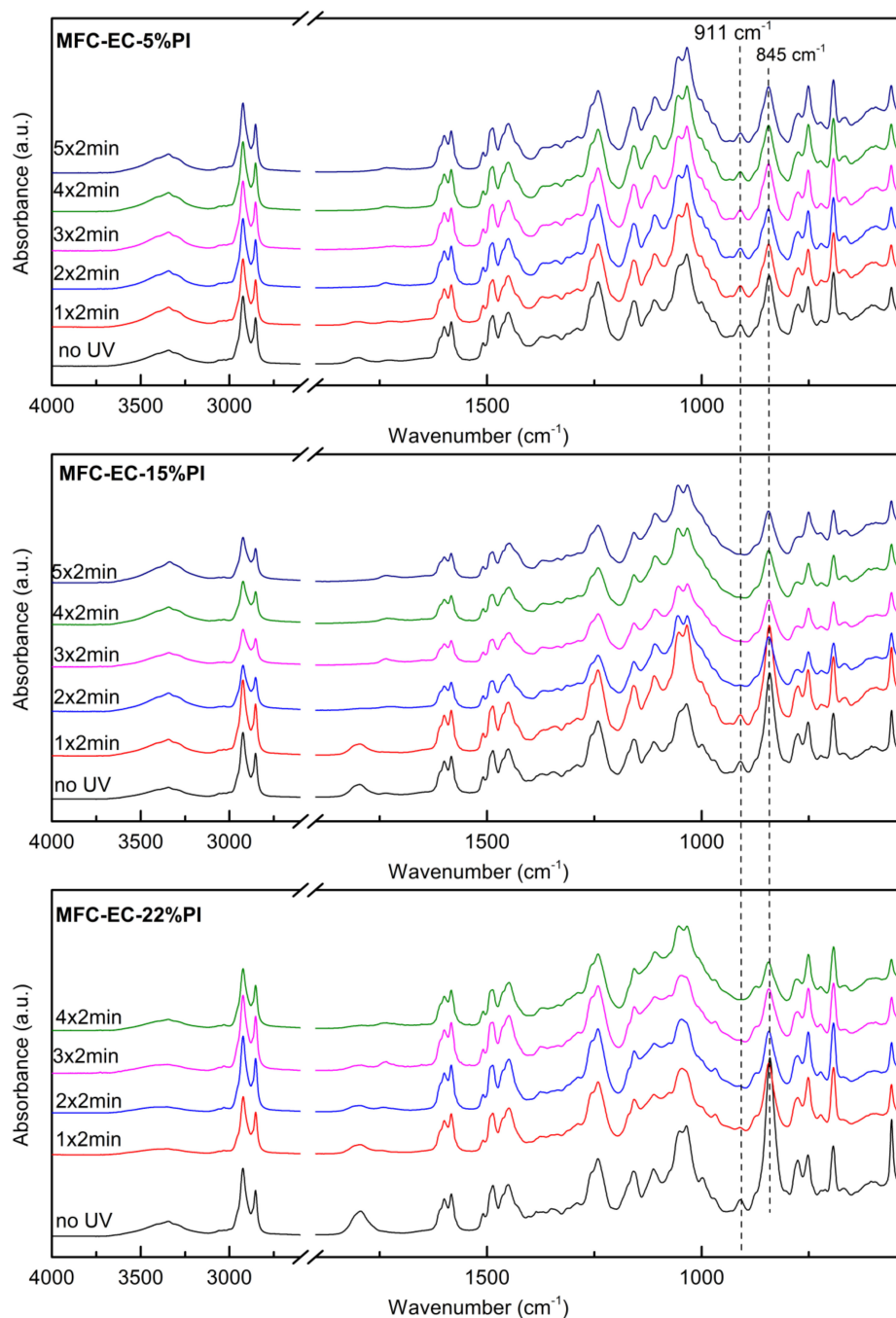
Figure 8. ATR FT-IR spectra composites MFC-EC-5%PI, MFC-EC-15%PI and MFC-EC-22%PI with different times of UV irradiation at 100\text{ mW cm}^{-2} ("n × 2 min" indicates that irradiation was carried out for n minutes on each side).
