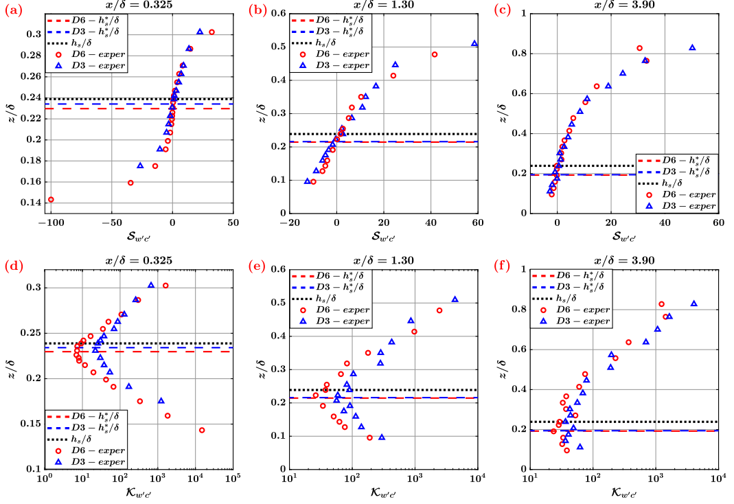
FIG. 3. Vertical profiles of (a)–(c) the skewness of wall-normal transport \mathcal{S}_{w'c'} , in linear-linear scale, and (d)–(f) the kurtosis \mathcal{K}_{w'c'} , in log-linear scale. The profiles are plotted at three streamwise locations, in the near field ( x/\delta = 0.325 ), in the far field ( x/\delta = 3.90 ), and at an intermediate location ( x/\delta = 1.30 ), for the two source diameters, D = 3 mm and D = 6 mm. The wall-normal coordinate of the source axis, h_s , is illustrated as a horizontal dotted line, while the plume axis height, h_s^* , is displayed as a blue (red) dashed line for the source D3 (D6).
