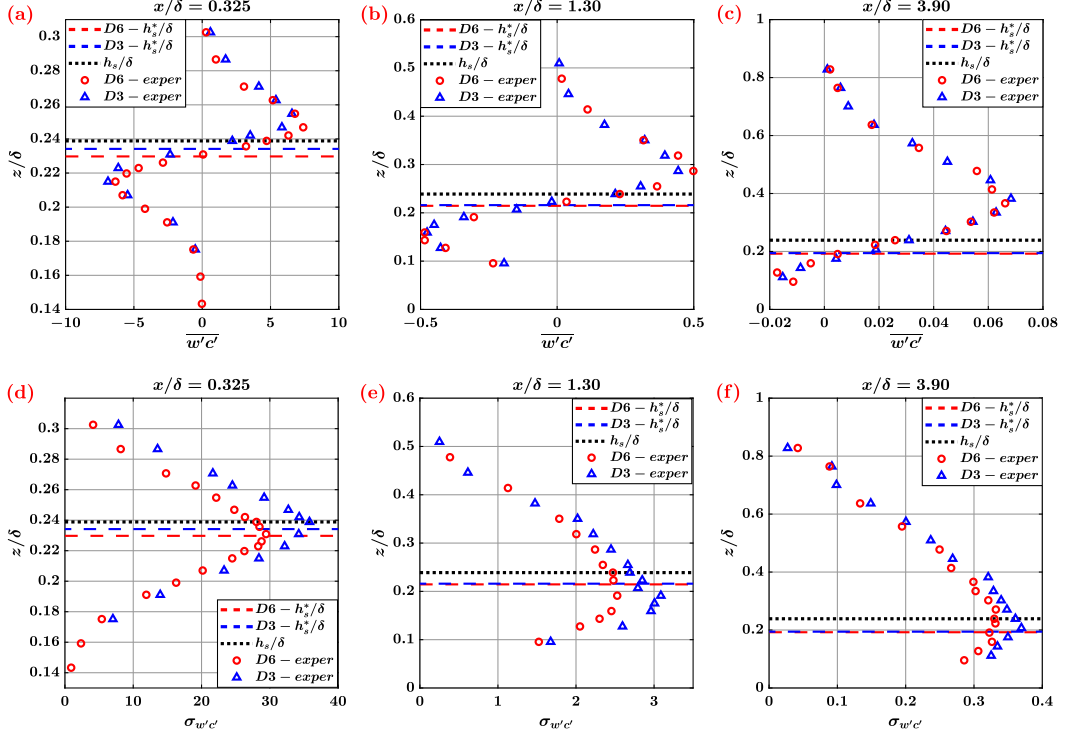
FIG. 2. Vertical profiles of (a)–(c) the mean value of wall-normal transport \overline{w'c'} and (d)–(f) the standard deviation \sigma_{w'c'} . The profiles are plotted at three streamwise locations, in the near field ( x/\delta = 0.325 ), in the far field ( x/\delta = 3.90 ), and at an intermediate location ( x/\delta = 1.30 ), for the two source diameters, D = 3 mm and D = 6 mm. The wall-normal coordinate of the source axis, h_s , is illustrated as a horizontal dotted line, while the plume axis height, h_s^* , is displayed as a blue (red) dashed line for the source D3 (D6).
