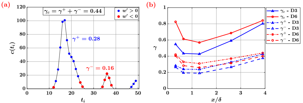
FIG. 5. (a) Example of the intermittent behavior of the concentration signal (first 50 values) measured at x/\delta = 1.30 and at the source axis. Blue and red data correspond to upward and downward transport, respectively. The corresponding values of the intermittency factor for the shown time interval are also reported. (b) Intermittency factors of the passive scalar concentration, \gamma_c , and wall-normal turbulent flux, \gamma^+ and \gamma^- , as a function of x/\delta along the source axis (i.e., y/\delta = 0 and z = h_s ).
