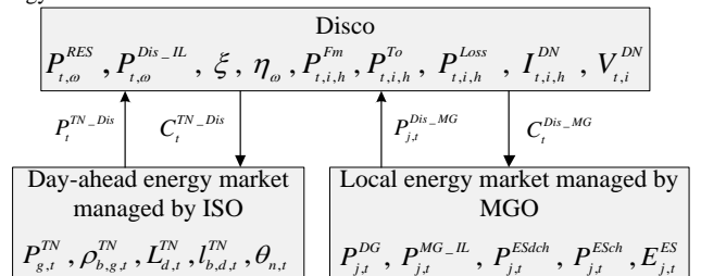
Fig. 2. The internal and external decision variables for each player in the proposed bi-level decision-making framework.
