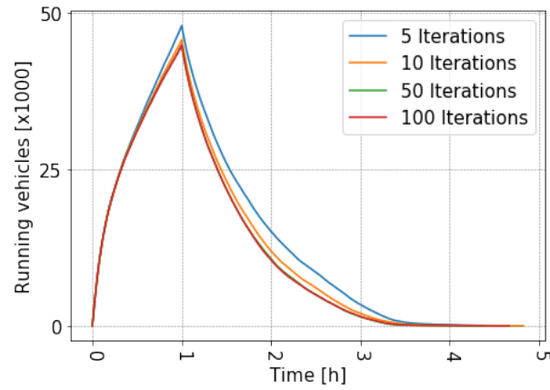
Fig. 6: Incremental Assignment.
