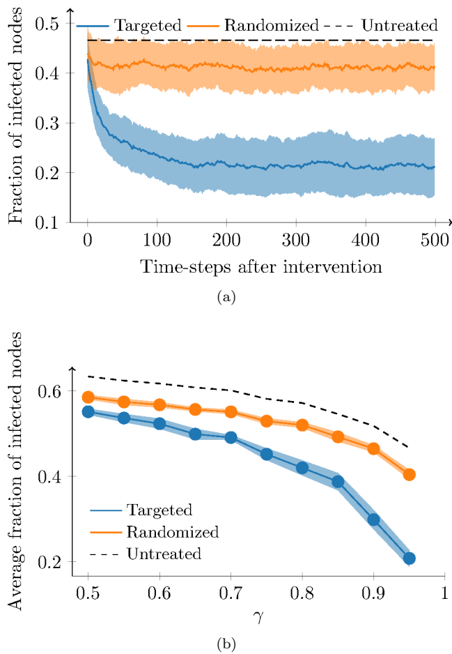
FIG. 7. Monte Carlo estimation over 100 runs of the effect of randomized (orange) and targeted (blue) immunization on the fraction of infected nodes. Dotted lines indicate the fraction of infected nodes in the absence of any immunization technique. In (a), we show the entire realizations for \gamma = 0.95 . The solid line is the average, while the light band is one standard deviation. In (b), we compare the average fraction of infected nodes for different values of \gamma . Bands identify 95% confidence intervals. Other parameters are n = 300 , \beta_d = \beta_a = -3 , \lambda = 0.9 , and \mu = 0.1 .
