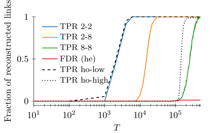
FIG. 5. Fraction of strong ties correctly identified by our algorithm for both heterogeneous and homogeneous backbones, and homogeneous activities a_i = 0.3 , for all the nodes. The other parameters are n = 200 , \gamma = 0.95 , \lambda = 0.9 , and \mu = 0.1 . Three cases for the backbone are examined: all the nodes have the same low-degree d_i = 2 (ho-low, dashed); all the nodes have the same high-degree d_i = 8 (ho-high, dotted); and half the nodes have d_i = 2 and half have d_i = 8 (he, colored). For the last case of heterogeneous degrees, the TPR curve is plotted with respect to links between nodes with low degree (blue), links between nodes of different degree (orange), and links between nodes with high degree (green). Only one FDR curve is plotted for all the cases, since they are practically indistinguishable (he, red).
