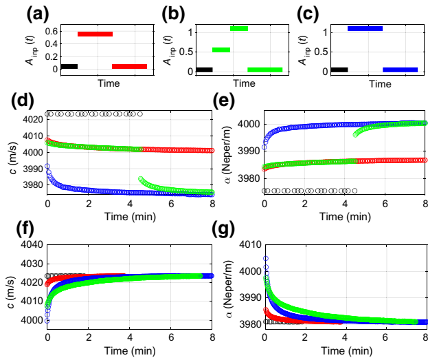
FIG. 6. Evolution of velocity and attenuation coefficient for sample B06 during conditioning for different experimental protocols. (a)–(c) Experimental protocols. Black symbols refer to preconditioning measurements, red symbols to conditioning at A_{\text{cnd}} = 0.58 V, blue symbols to conditioning at A_{\text{cnd}} = 1.2 V, and green symbols to conditioning at successively increasing conditioning amplitudes. (d) and (e) Conditioning measurements. (f) and (g) Relaxation measurements.
