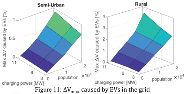
Figure 11: \Delta V_{\max} caused by EVs in the grid
