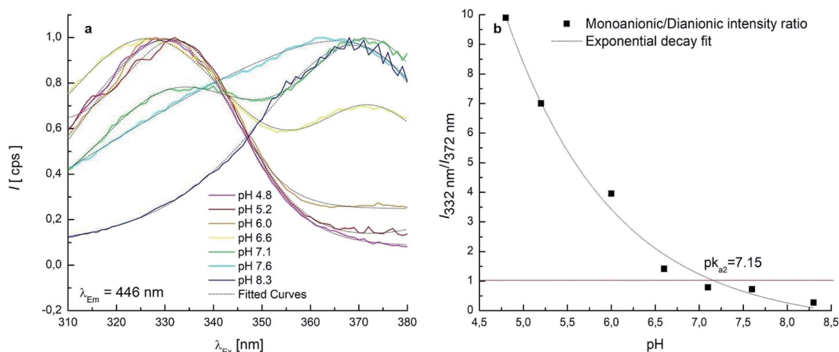
Fig. 5 (a) Excitation spectra collected at fixed \lambda_{\text{Em}} = 446 \text{ nm} in the pH range 4.8–8.3 (normalised intensity scale and Gaussian fitted curves); (b) monoanionic/dianionic intensity I_{332} to I_{372} ratio as a function of the solution pH.
