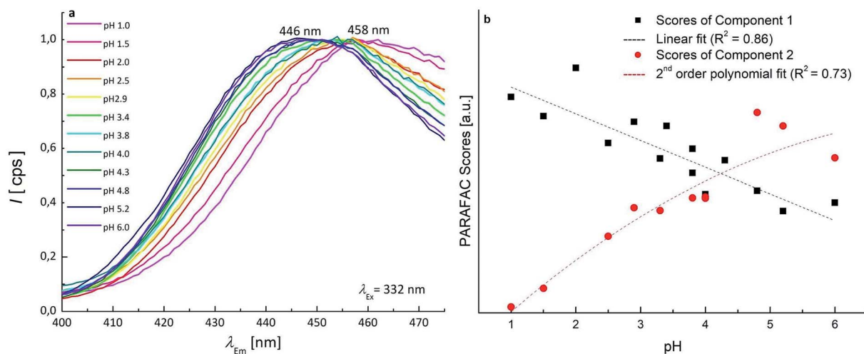
Fig. 4 (a) Experimental emission spectra of OTA 1.24 \times 10^{-7} \text{ mol L}^{-1} in the pH range 1.0–6.0 (normalised intensity scale); (b) scatter scores plot as a function of pH, the scores of the two components of PARAFAC model are shown.
