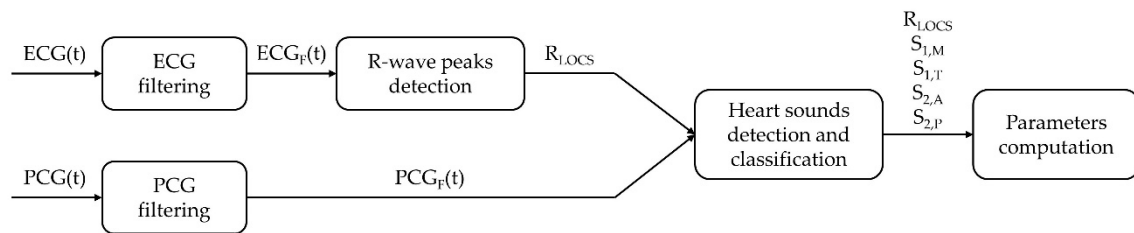
Figure 3. Block diagram of the overall processing.
